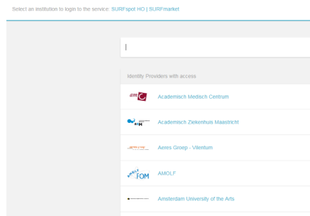
Figure 11: SURFconext screenshot
