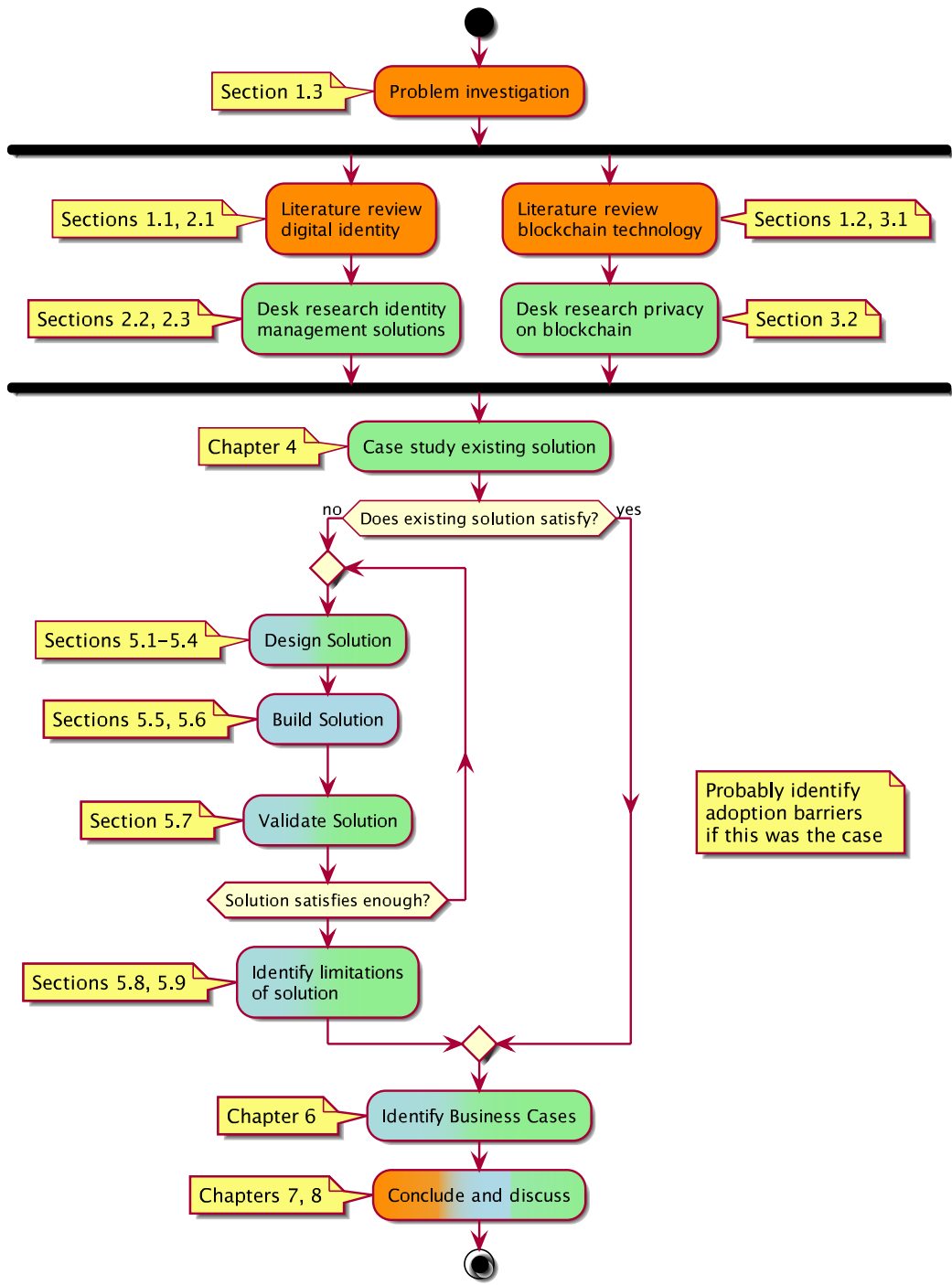
Figure 5: Research Design
