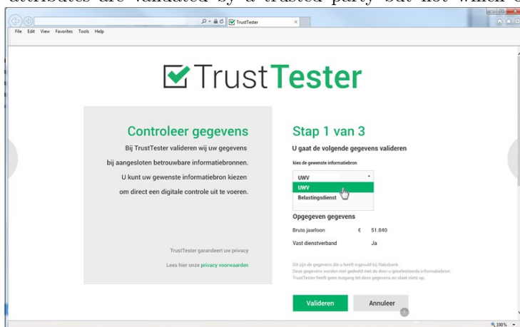
Figure 10: Screenshot TrustTester
